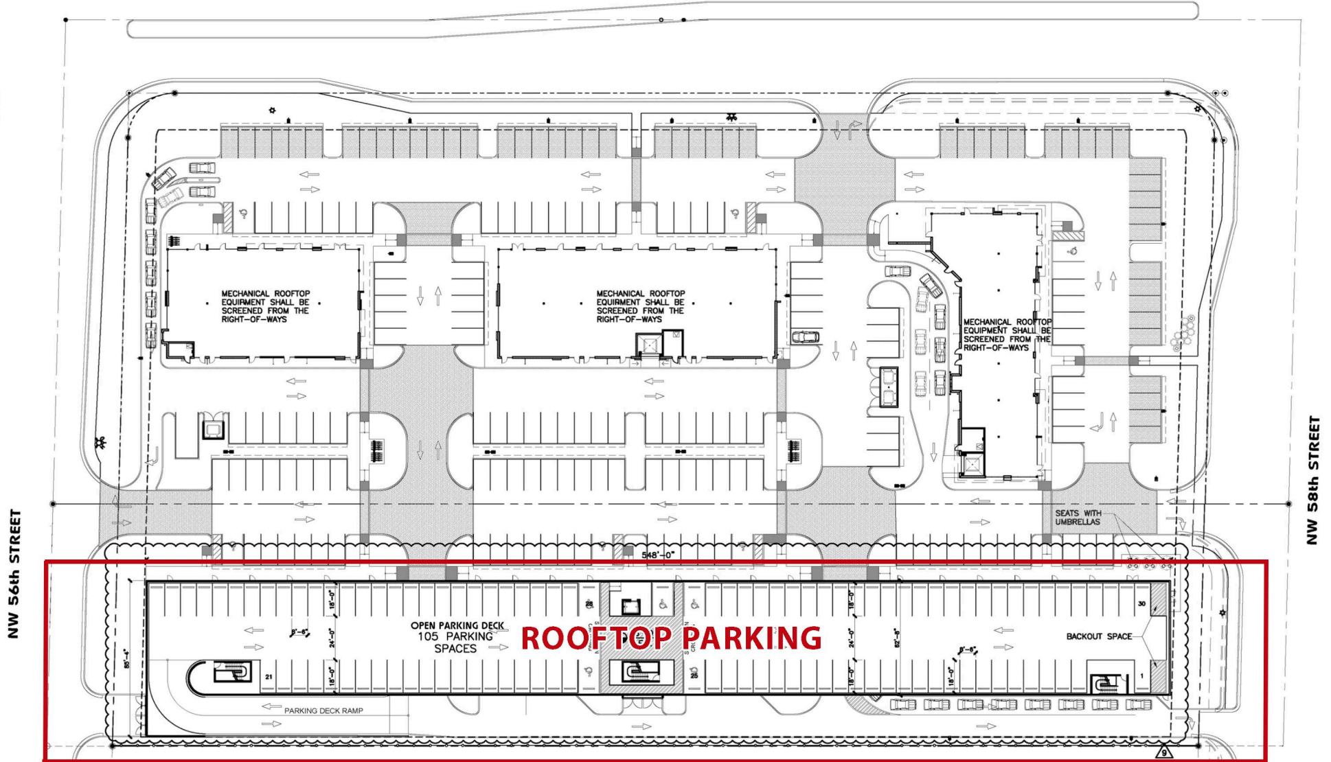
16 Level 2 Parking Deck SCALE 1"=30'-0"
